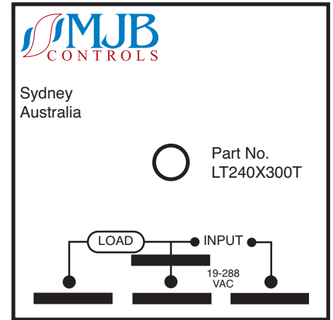
LT240X300T Anti Cycle Timer
